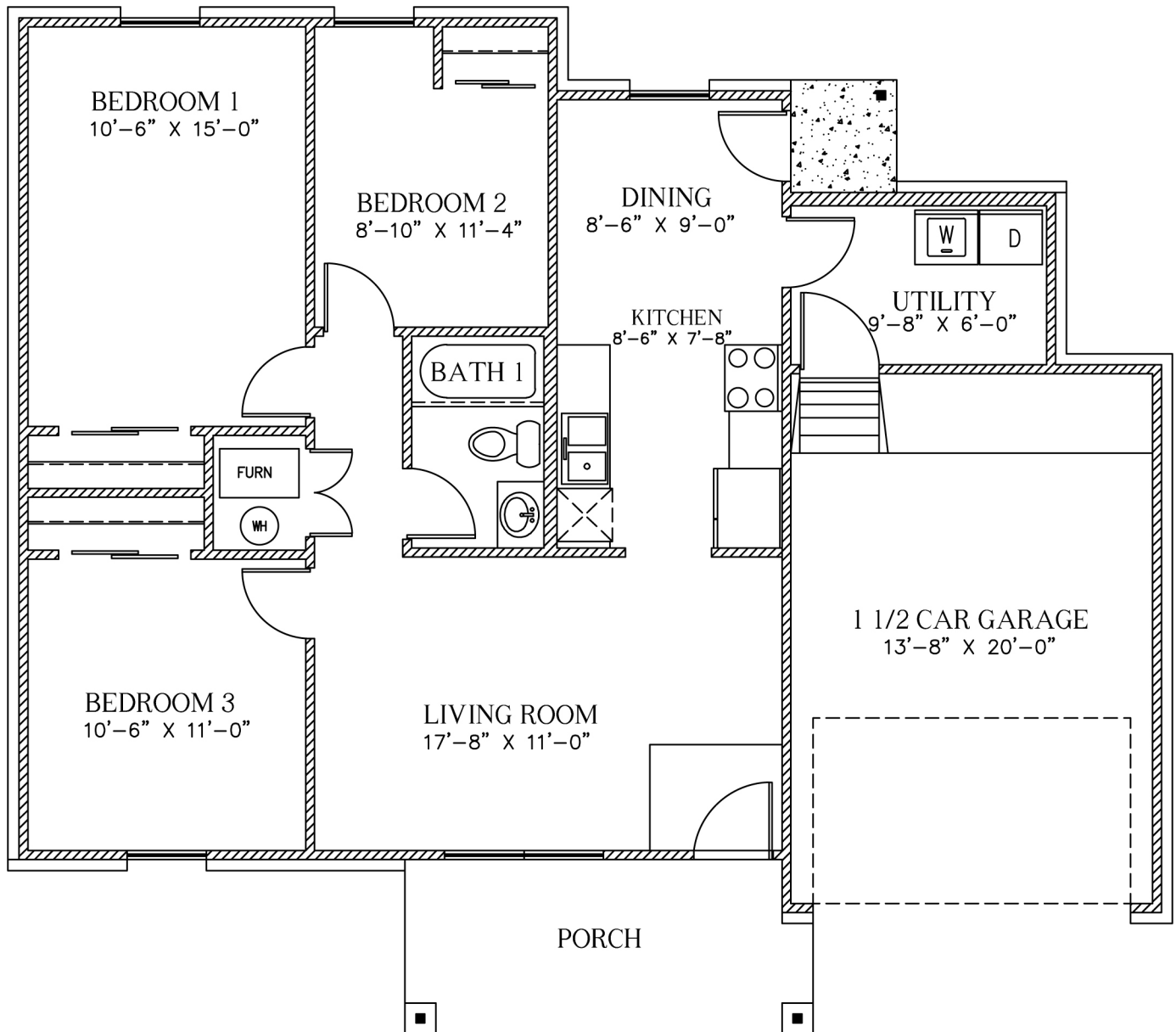
1013 FLOOR PLAN
