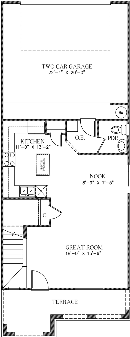
1765A - FIRST FLOOR
