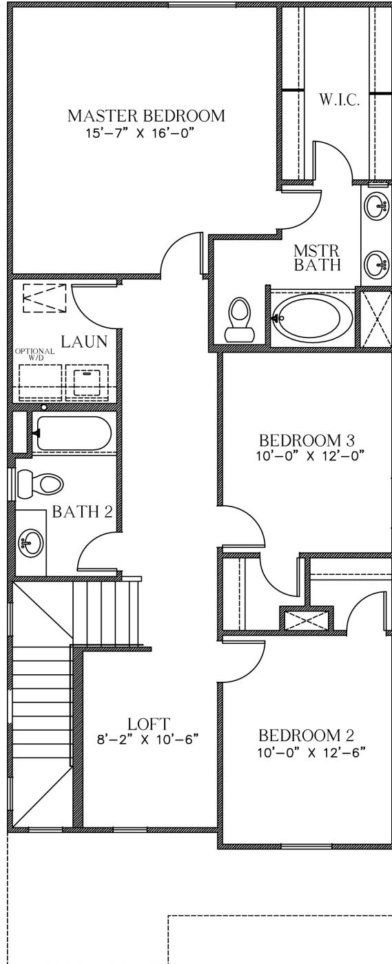
1765A - SECOND FLOOR
