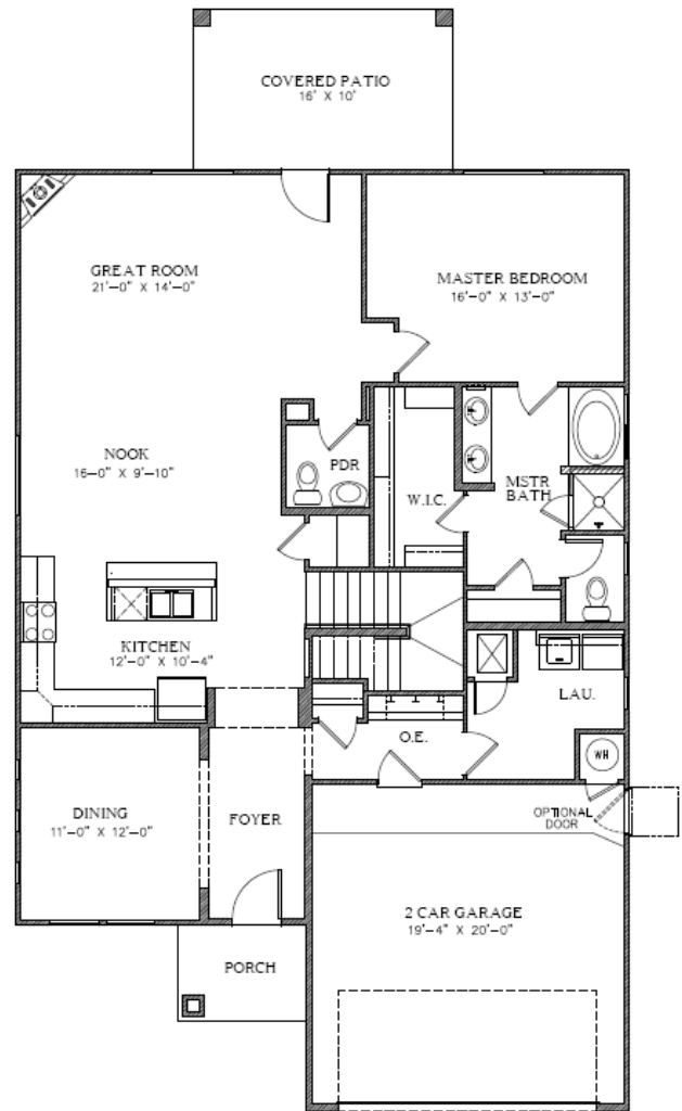
7765 1ST FLOOR PLAN
